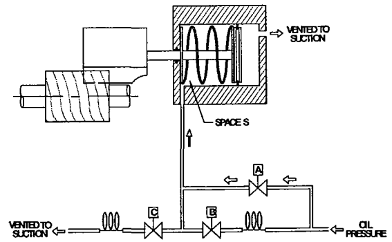
FIGURE 2-7: Minimum Capacity
