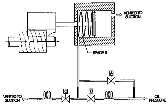
FIGURE 2-10: Load Constant
