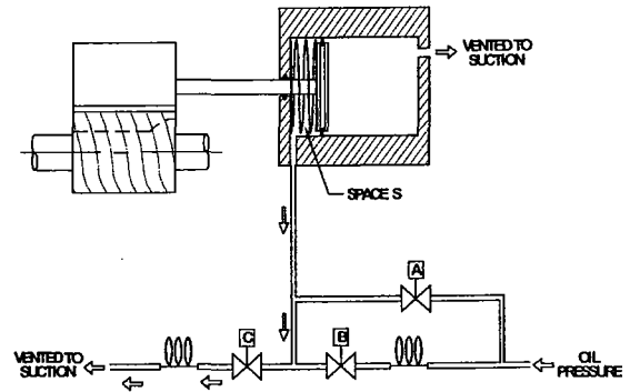
FIGURE 2-8: Loading Up
