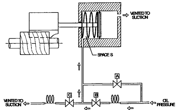
FIGURE 2-9: Unloading
