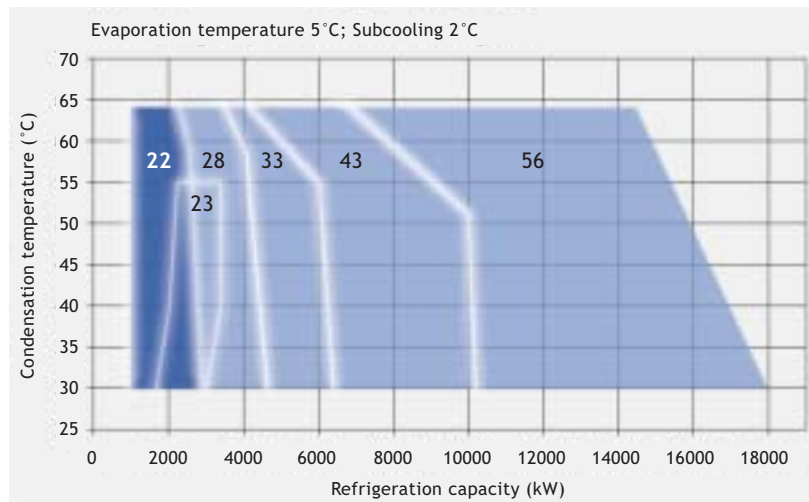
Uniturbo® range of compressors, marked in dark blue the data for Uniturbo® 22
