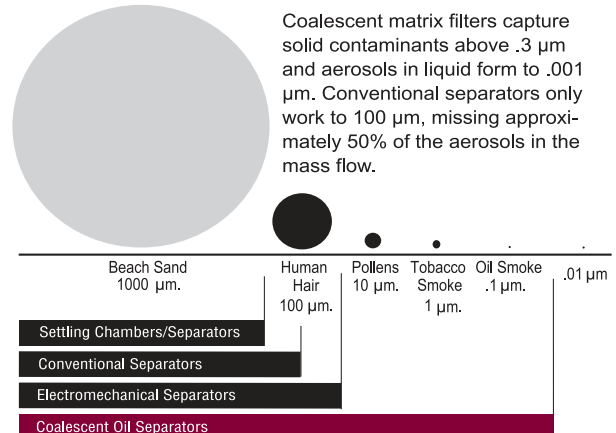
Illustration #4: Coalescent Oil Separator Filtration Level
