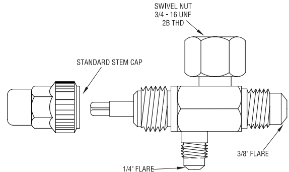
Rotalock Valve
