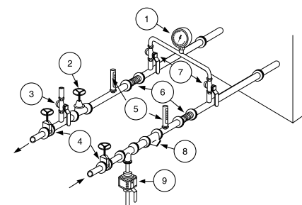
Figure 6 - Unit without hydraulic module and buffer tank - typical water circuit
